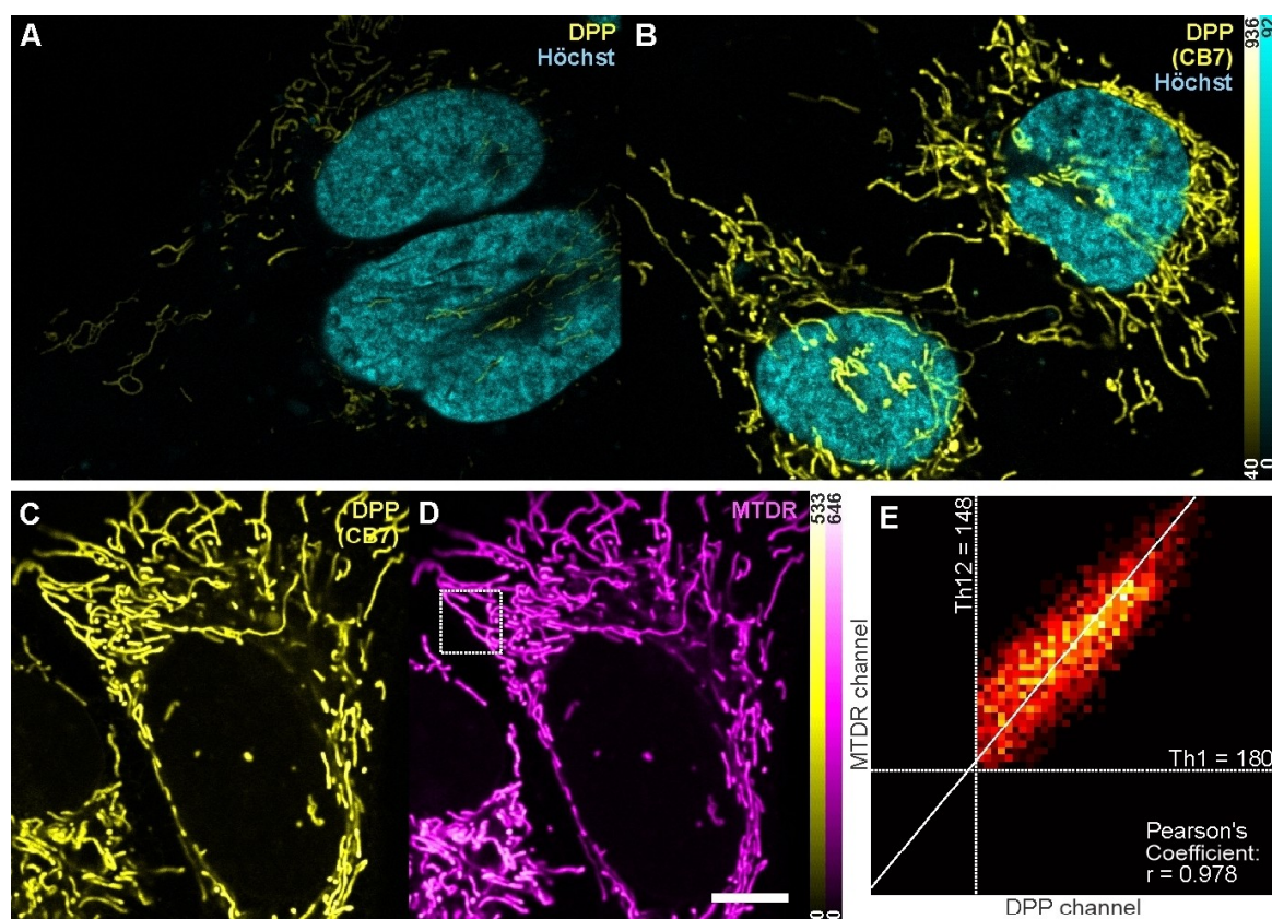
Figure 3. Confocal images of live U2OS cells. Cells were co-labelled with nuclear stain Hoechst dye and 1 μM DPP without CB7 (A) and DPP pre-mixed with CB7 1 mM (B). (C, D) Cells were simultaneously stained with pre-mixed 1 μM DPP+CB7 1 mM and MitoTracker Deep Red FM; (E) Corresponding colocalization 2D histogram. Scale bar: 10 μm.
